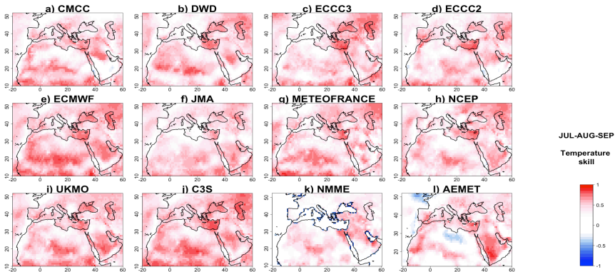
Figure 7: Temperature correlations in forecast, compared to observations, for the three seasonal forecast systems C3S (j) and NMME (k) and AEMET (l). Higher values indicate better model predictive skill. From (a) to (i) models of the C3S ensemble
