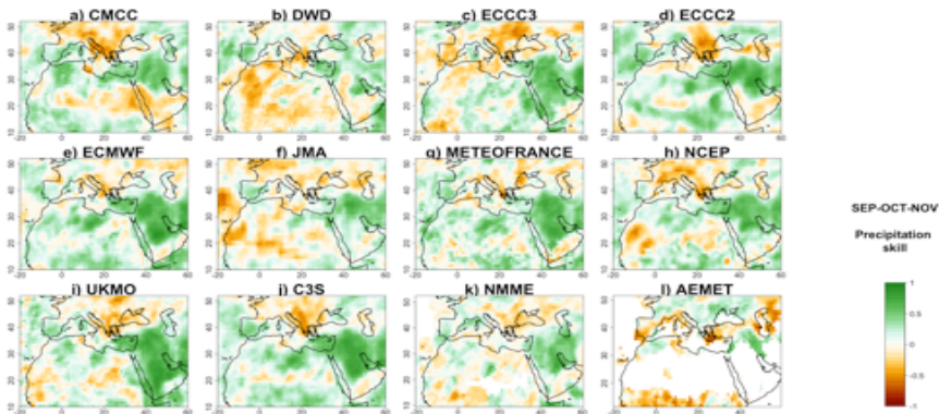
Figure 6: Precipitation correlations in SON forecast, compared to observations, for the three seasonal forecast systems C3S (j), NMME (k) and AEMET(l). Higher values indicate better model predictive skill. From (a) to (i) models of the C3S ensemble.
