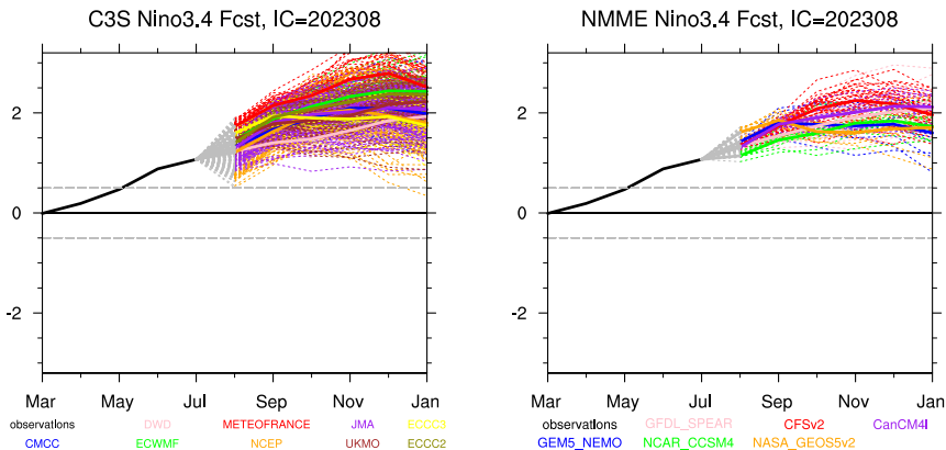
Figure 1: Niño3.4 prediction from all the ensemble members of the C3S multi-system (a) and the NMME multi-system (b), for the start-date of Aug.
