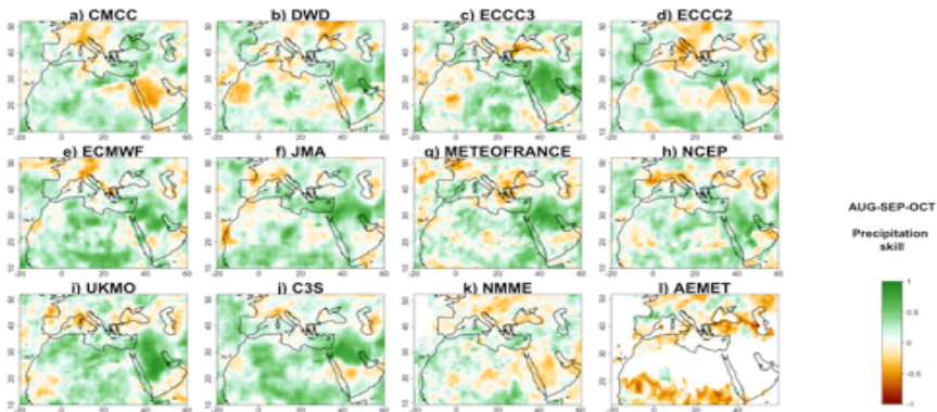
Figure 6: Precipitation correlations in ASO forecast, compared to observations, for the three seasonal forecast systems C3S (j), NMME (k) and AEMET(l). Higher values indicate better model predictive skill. From (a) to (i) models of the C3S ensemble.
