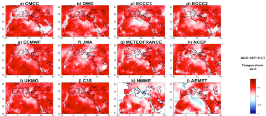
Figure 7: Temperature correlations in ASO forecast, compared to observations, for the three seasonal forecast systems C3S (j) and NMME (k) and AEMET(l). Higher values indicate better model predictive skill. From (a) to (i) models of the C3S ensemble
