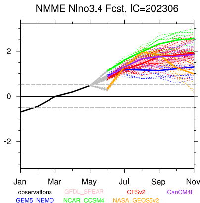
Figure 1: Niño3.4 prediction from all the ensemble members of the C3S multi-system (a) and the NMME multi-system (b), for the start-date of Jun.
