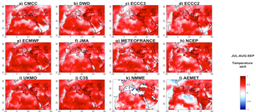
Figure 7: Temperature correlations in JAS forecast, compared to observations, for the three seasonal forecast systems C3S (j) and NMME (k) and AEMET(l). Higher values indicate better model predictive skill. From (a) to (i) models of the C3S ensemble
