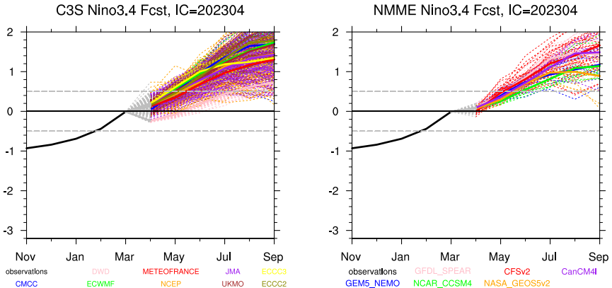
Figure 1: Niño3.4 prediction from all the ensemble members of the C3S multi-system (a) and the NMME multi-system (b), for the start-date of Apr.
