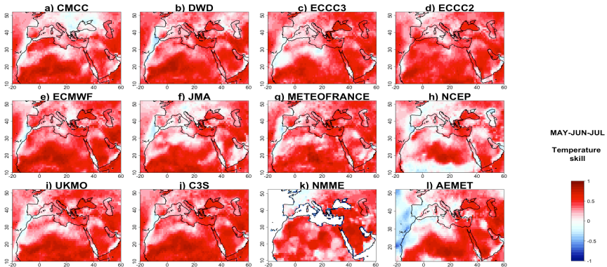
Figure 7: Temperature correlations in MJJ forecast, compared to observations, for the three seasonal forecast systems C3S (j) and NMME (k) and AEMET(l). Higher values indicate better model predictive skill. From (a) to (i) models of the C3S ensemble
