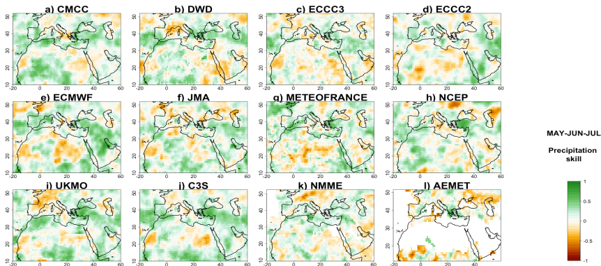
Figure 6: Precipitation correlations in MJJ forecast, compared to observations, for the three seasonal forecast systems C3S (j), NMME (k) and AEMET(l). Higher values indicate better model predictive skill. From (a) to (i) models of the C3S ensemble.
