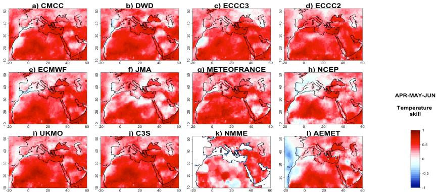
Figure 7: Temperature correlations in AMJ forecast, compared to observations, for the three seasonal forecast systems C3S (j) and NMME (k) and AEMET(l). Higher values indicate better model predictive skill. From (a) to (i) models of the C3S ensemble
