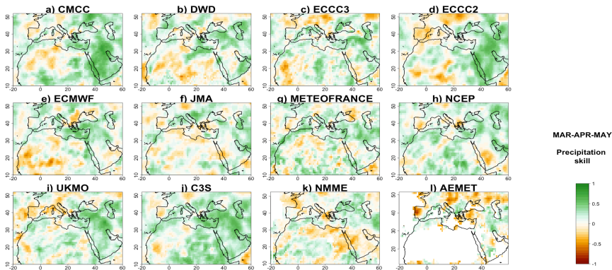
Figure 6: Precipitation correlations in MAM forecast, compared to observations, for the three seasonal forecast systems C3S (j), NMME (k) and AEMET(l). Higher values indicate better model predictive skill. From (a) to (i) models of the C3S ensemble.
