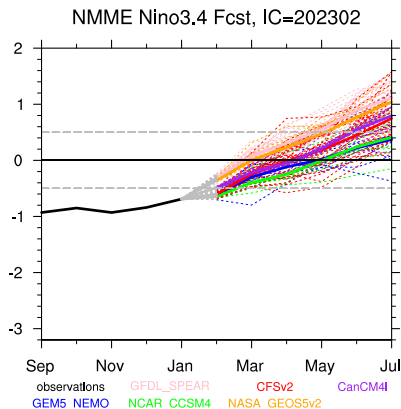
Figure 1: Niño3.4 prediction from all the ensemble members of the C3S multi-system (a) and the NMME multi-system (b), for the start-date of Feb.
