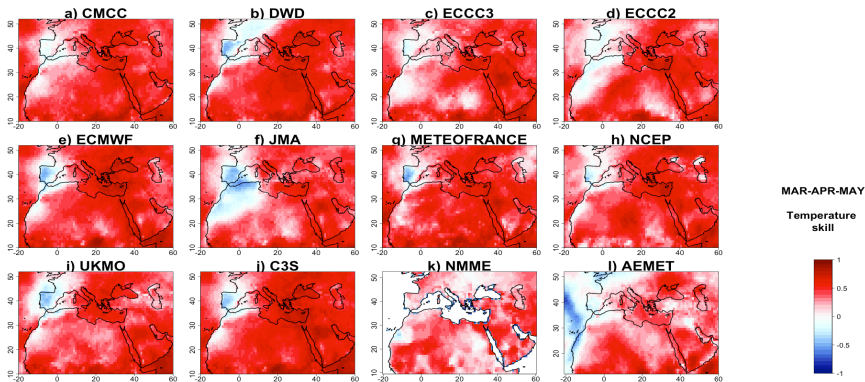
Figure 7: Temperature correlations in MAM forecast, compared to observations, for the three seasonal forecast systems C3S (j) and NMME (k) and AEMET(l). Higher values indicate better model predictive skill. From (a) to (i) models of the C3S ensemble
