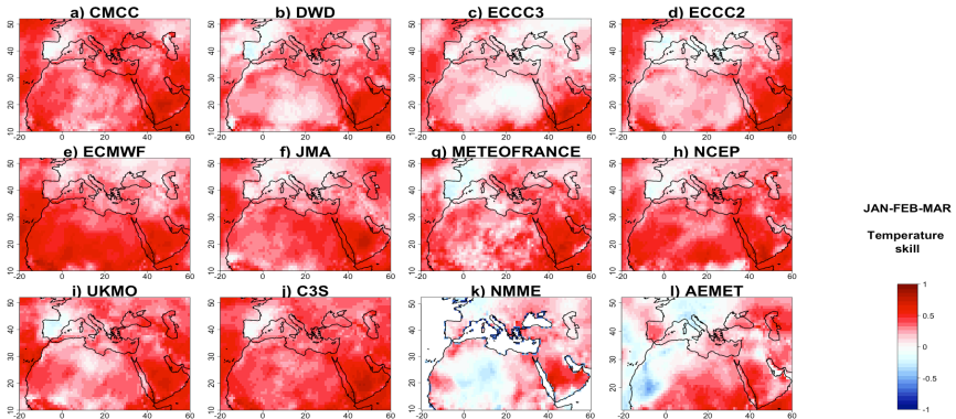
Figure 7: Temperature correlations in JFM forecast, compared to observations, for the three seasonal forecast systems C3S (j) and NMME (k) and AEMET(l). Higher values indicate better model predictive skill. From (a) to (i) models of the C3S ensemble
