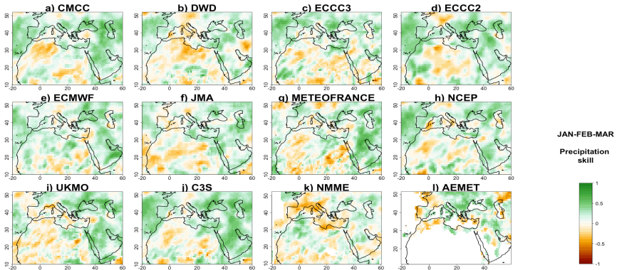
Figure 6: Precipitation correlations in JFM forecast, compared to observations, for the three seasonal forecast systems C3S (j), NMME (k) and AEMET(l). Higher values indicate better model predictive skill. From (a) to (i) models of the C3S ensemble.
