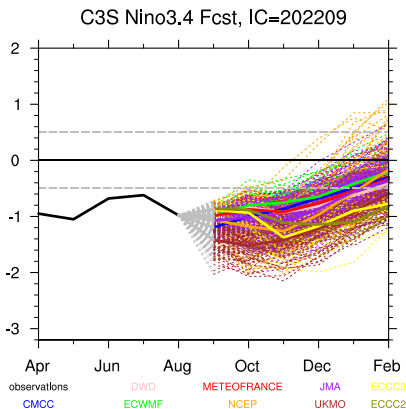
Figure 1: Niño3.4 prediction from all the ensemble members of the C3S multi-system (a) and the NMME multi-system (b), for the start-date of Sep.
