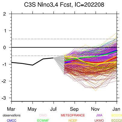
Figure 1: Niño3.4 prediction from all the ensemble members of the C3S multi-system (a) and the NMME multi-system (b), for the start-date of Aug.
