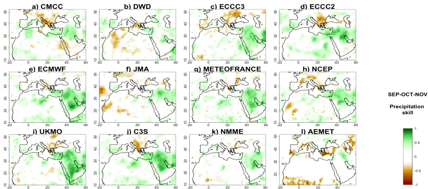
Figure 6: Precipitation correlations in forecast, compared to observations, for the three seasonal forecast systems C3S (j), NMME (k) and AEMET(l). Higher values indicate better model predictive skill. From (a) to (i) models of the C3S ensemble.
