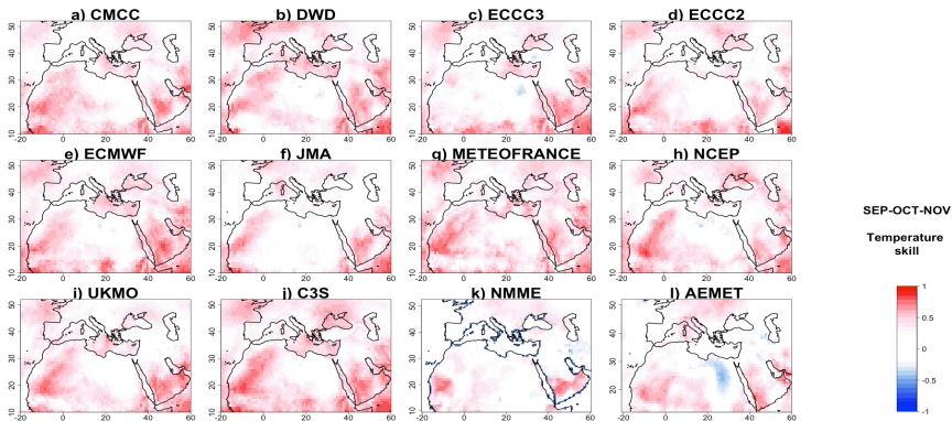
Figure 7: Temperature correlations in forecast, compared to observations, for the three seasonal forecast systems C3S (j) and NMME (k) and AEMET(l). Higher values indicate better model predictive skill. From (a) to (i) models of the C3S ensemble
