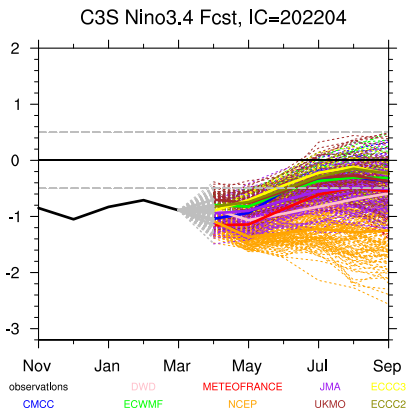
Figure 1: Niño3.4 prediction from all the ensemble members of the C3S multi-system (a) and the NMME multi-system (b), for the start-date of Apr.
