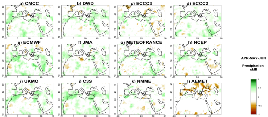
Figure 6: Precipitation correlations in forecast, compared to observations, for the three seasonal forecast systems C3S (j), NMME (k) and AEMET (l). Higher values indicate better model predictive skill. From (a) to (i) models of the C3S ensemble.
