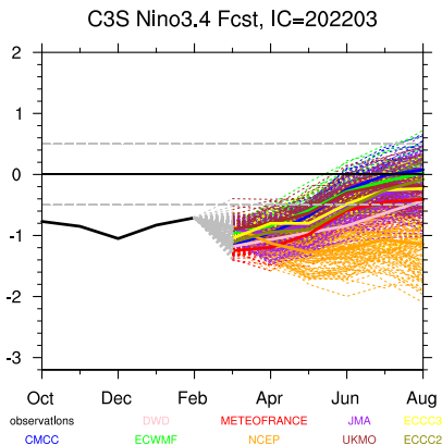
Figure 1: Niño3.4 prediction from all the ensemble members of the C3S multi-system (a) and the NMME multi-system (b), for the start-date of Mar.
