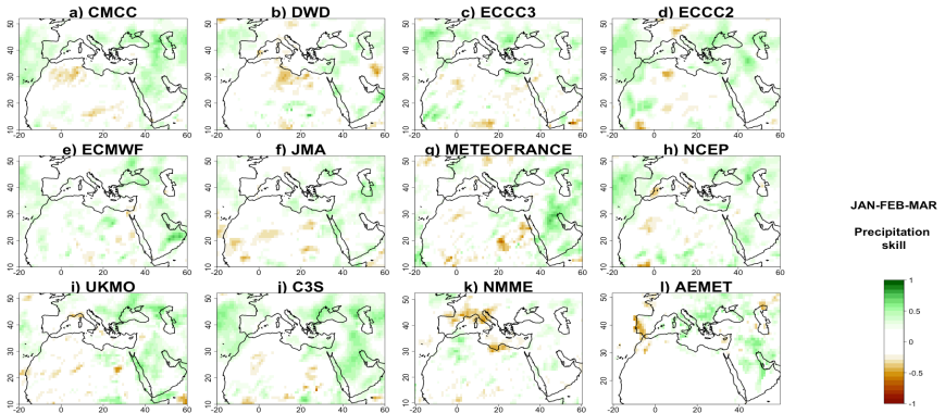
Figure 6: Precipitation correlations in forecast, compared to observations, for the three seasonal forecast systems C3S (j), NMME (k) and AEMET(l). Higher values indicate better model predictive skill. From (a) to (i) models of the C3S ensemble.
