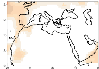
Colder
