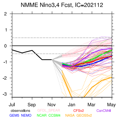
Figure 1: Niño3.4 prediction from all the ensemble members of the C3S multi-system (a) and the NMME multi-system (b), for the start-date of Dec.
