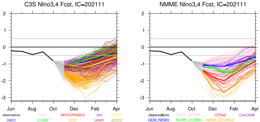
Figure 1: Niño3.4 prediction from all the ensemble members of the C3S multi-system (a) and the NMME multi-system (b), for the start-date of Nov.
