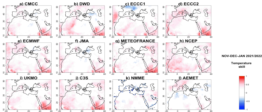
Figure 5: Temperature correlations in forecast, compared to observations, for the three seasonal forecast systems C3S (j) and NMME (k) and AEMET (l). Higher values indicate better model predictive skill. From (a) to (i) models of the C3S ensemble
