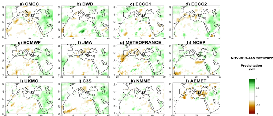
Figure 3: Precipitation correlations in forecast, compared to observations, for the three seasonal forecast systems C3S (j), NMME (k) and AEMET(l). Higher values indicate better model predictive skill. From (a) to (i) models of the C3S ensemble.
