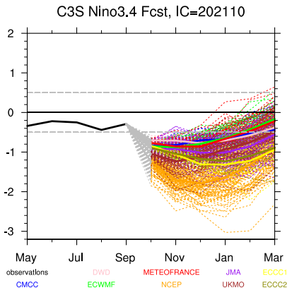
Figure 1: Niño3.4 prediction from all the ensemble members of the C3S multi-system (a) and the NMME multi-system (b), for the start-date of Oct.
