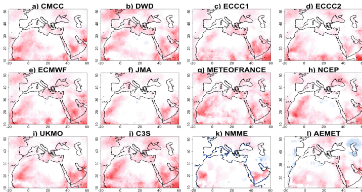
Figure 5: Temperature correlations in forecast, compared to observations, for the three seasonal forecast systems C3S (j) and NMME (k) and AEMET(l). Higher values indicate better model predictive skill. From (a) to (i) models of the C3S ensemble
