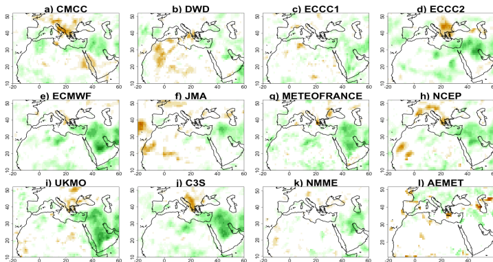
Figure 3: Precipitation correlations in forecast, compared to observations, for the three seasonal forecast systems C3S (j), NMME (k) and AEMET(l). Higher values indicate better model predictive skill. From (a) to (i) models of the C3S ensemble.
