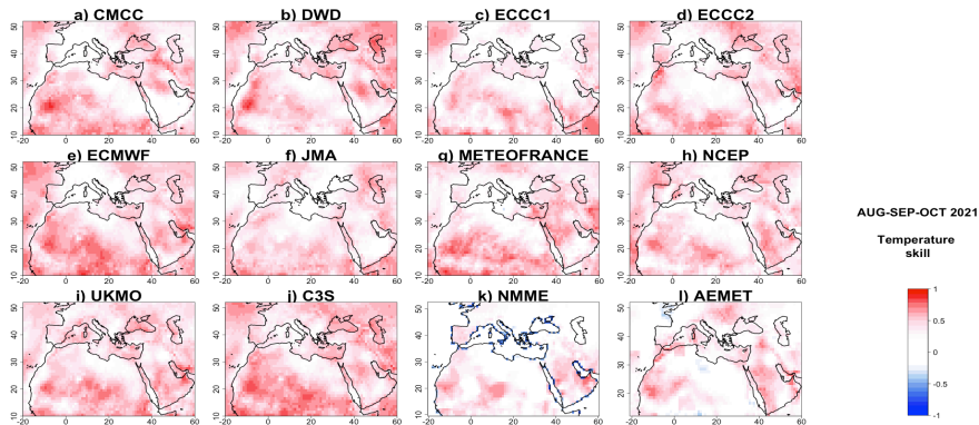
Figure 5: Temperature correlations in forecast, compared to observations, for the three seasonal forecast systems C3S (j) and NMME (k) and AEMET(l). Higher values indicate better model predictive skill. From (a) to (i) models of the C3S ensemble
