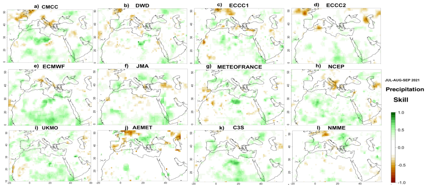
Figure 3: Precipitation correlations in July-August-September forecast, compared to observations, for the three seasonal forecast systems AEMET(j), C3S (k), NMME (l). Higher values indicate better model predictive skill. From (a) to (i) models of the C3S ensemble.
