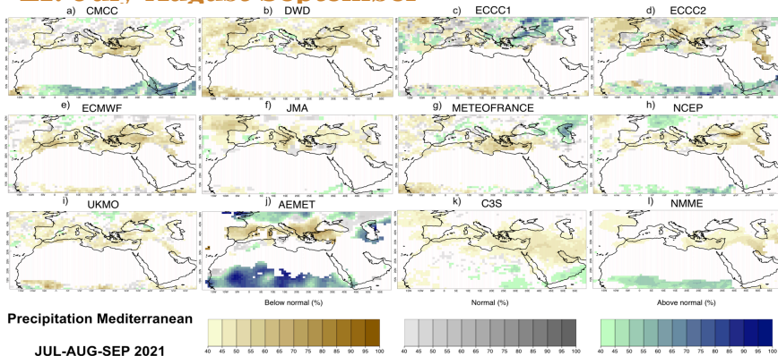
Figure 2: Most likely tercile of Precipitation in the three seasonal forecast systems AEMET(j), C3S (k), NMME (l) and in July-August-September (L1) forecast. From (a) to (i) models of the C3S ensemble.
