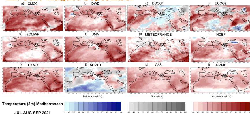
Figure 4: Most likely tercile of Temperature in the three seasonal forecast systems AEMET(j), C3S (k) and NMME (l) in July-August-September (L1) forecast. From (a) to (i) models of the C3S ensemble
