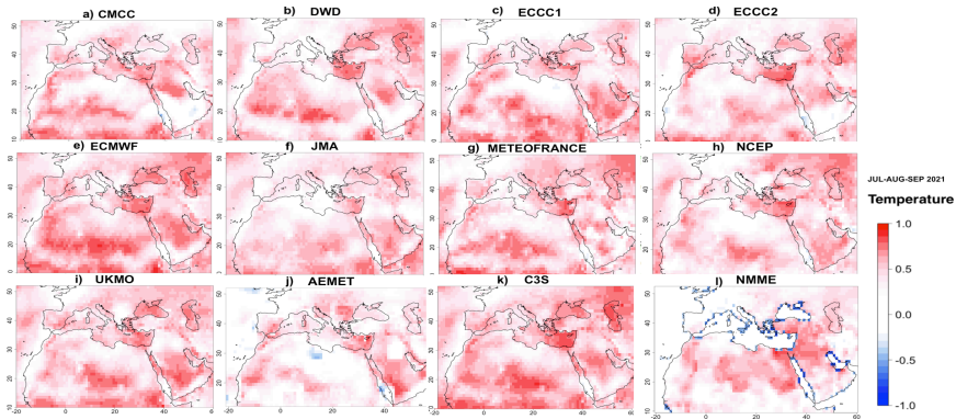
Figure 5: Temperature correlations in July-August-September forecast, compared to observations, for the three seasonal forecast systems AEMET(j), C3S (k) and NMME (l). Higher values indicate better model predictive skill. From (a) to (i) models of the C3S ensemble
