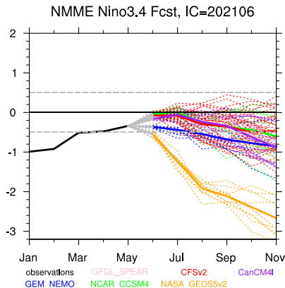
Figure 1: Niño3.4 prediction from all the ensemble members of the C3S multi-system (a) and the NMME multi-system (b), for the start-date of June.
